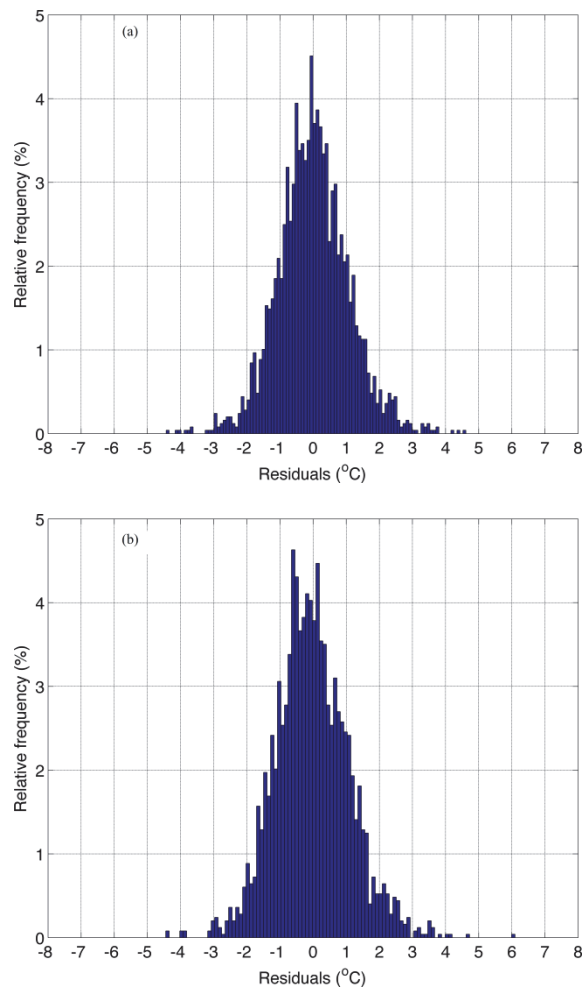
Figure 3: The residuals' distribution for the (a) MLPANN and the (b) RBFANN models.
