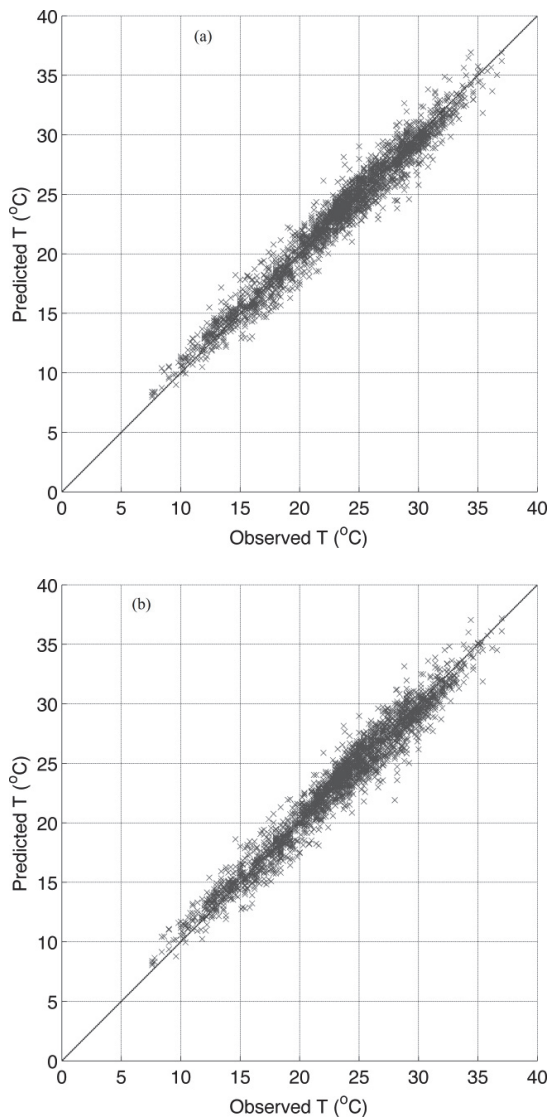
Figure 2: Comparison of the observed and predicted air temperature values for the (a) MLPANN and (b) RBFANN schemes.
