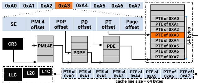
Fig. 1: Page table locality on a x86-64 page table walk.
