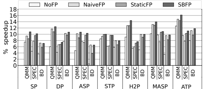
Fig. 8: Performance impact of free TLB prefetching scenarios.
