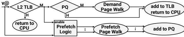
Fig. 2: System with TLB prefetching. Diamonds indicate decision points, circles indicate actions.
